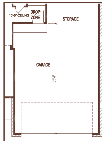
3'-0" GARAGE EXTENSION
