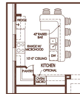
EXTENDED ISLAND 1
