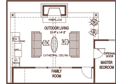
OUTDOOR LIVING
