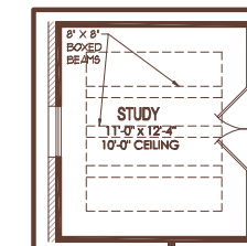
CEILING BEAM DETAIL AT STUDY
