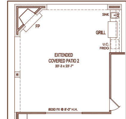
OUTDOOR LIVING
