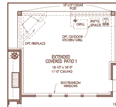
EXTENDED COVERED PATIO 1
