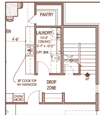
STAIRS AT FIRST FLOOR FOR BEDROOM 6 OR BONUS ROOM
